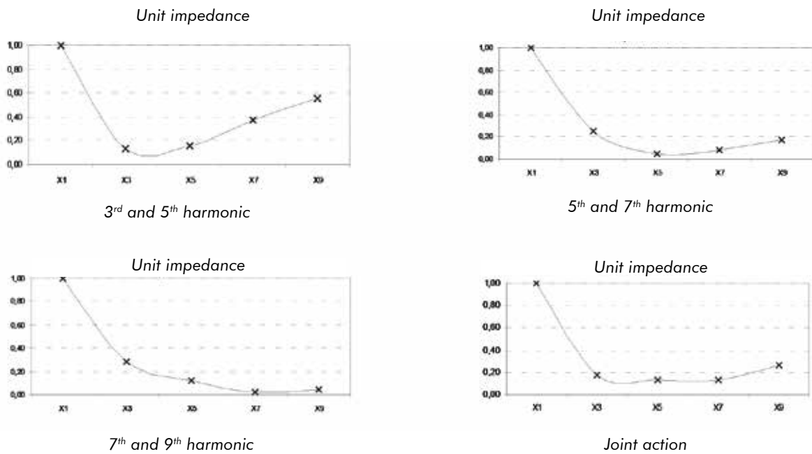
Figure 6. Several different ECONELEC® equipment filtering solutions.
