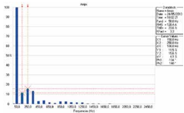
Figure 2. FFT waveform of current in typical GLVB.
