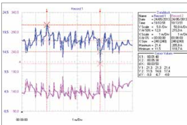
Figure 1. Waveform of current in typical GLVB (General Low Voltage Boards).
