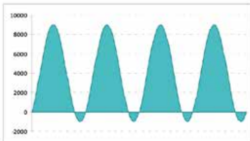
S = 5 \text{ kVA}, P = 4 \text{ kW}
